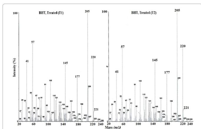
Figure 2: GC-MS spectra of treated butylatedhydroxytoluene sample T1 and T2.
