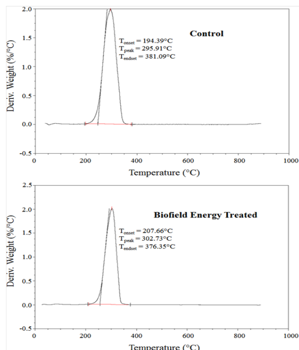
Figure 4: DTG thermograms of the control and Biofield Energy Treated Polylactic-co-glycolic acid
