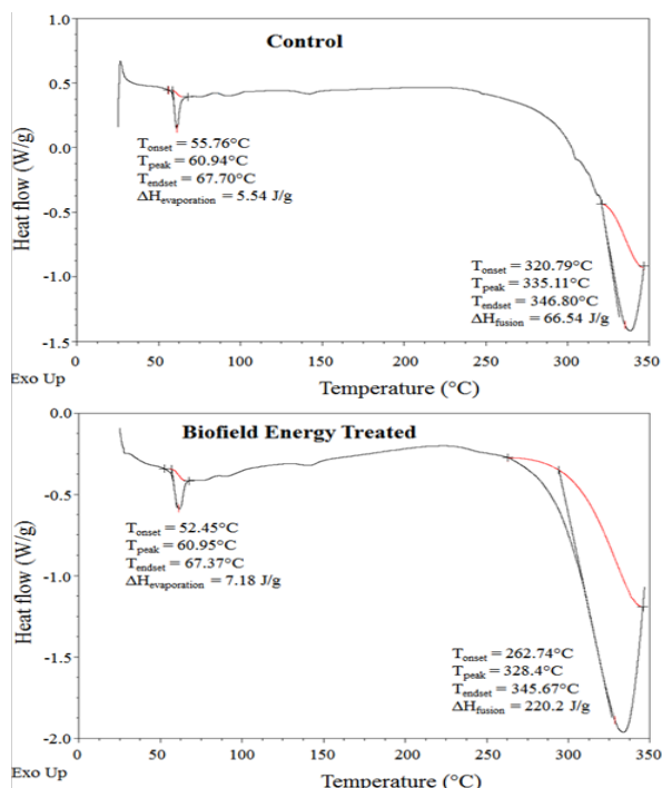
Figure 2: DSC thermograms of the control and Biofield Energy Treated Polylactic-co-glycolic acid
