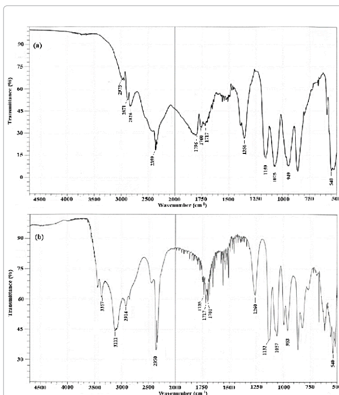
Figure 2: FT-IR spectra of disodium hydrogen orthophosphate (a) control and (b) treated.
